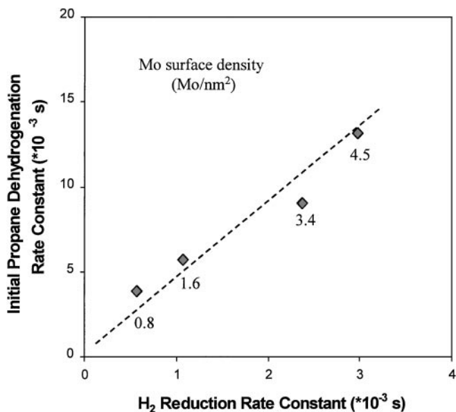
FIG. 10. Dependence of initial propene formation rate constant at 703 K on H 2 reduction rate constant at 673 K for MoO x /Al 2 O 3 catalysts.
